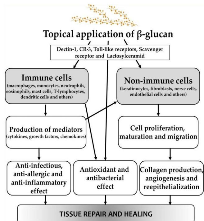
Figure 13: Schematic depiction of \beta -glucan pluripotent mechanisms in wound healing [157].
