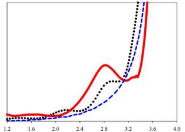
Figure 3: Extinction coefficient of Cadmium Oxide (CdO) thin films with Cd concentrations of (a) 0.5%, (b) 1%, (c) 1.5% and (p) pure sample.
